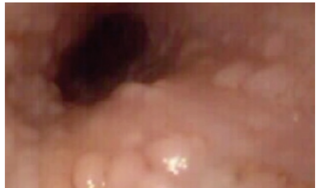
Figure 5. Nodular esophagitis
