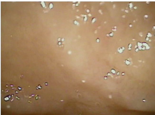
Figure 17. Non-specific duodenitis
